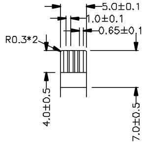
DETAIL A SCALE 2.0
